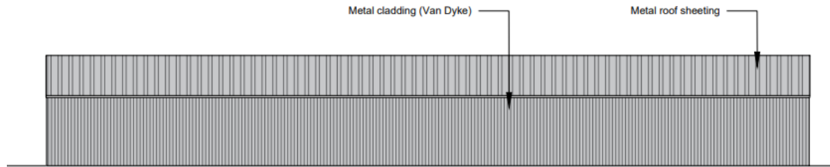
South Elevations
